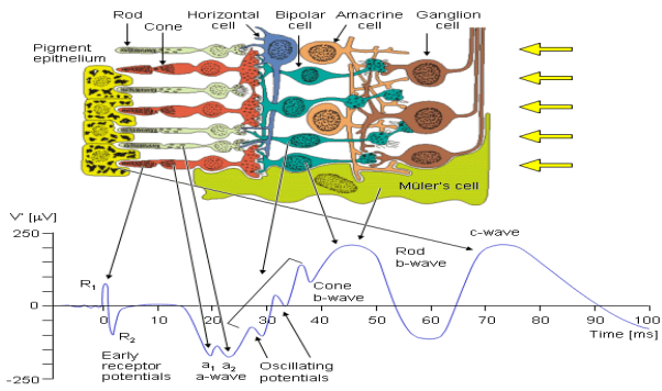
Figure 2. Signal is produced by initial changes in photo pigment molecule of the receptor considering light action
