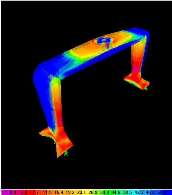
Figure 15. Optimized frame model using SAP software
