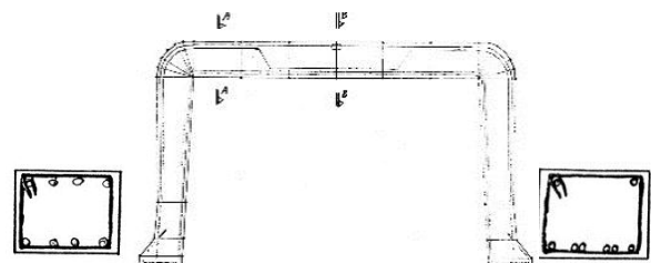
Figure 11. Reinforcement of the optimal frame
