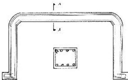
Figure 9. Reinforcement of the original frame
