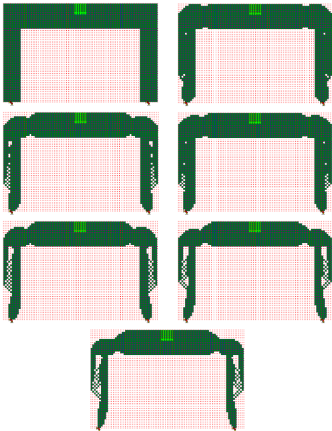
Figure 13. Display the stages of geometric frame optimization
