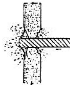
Figure 3. Local effect of perforation
