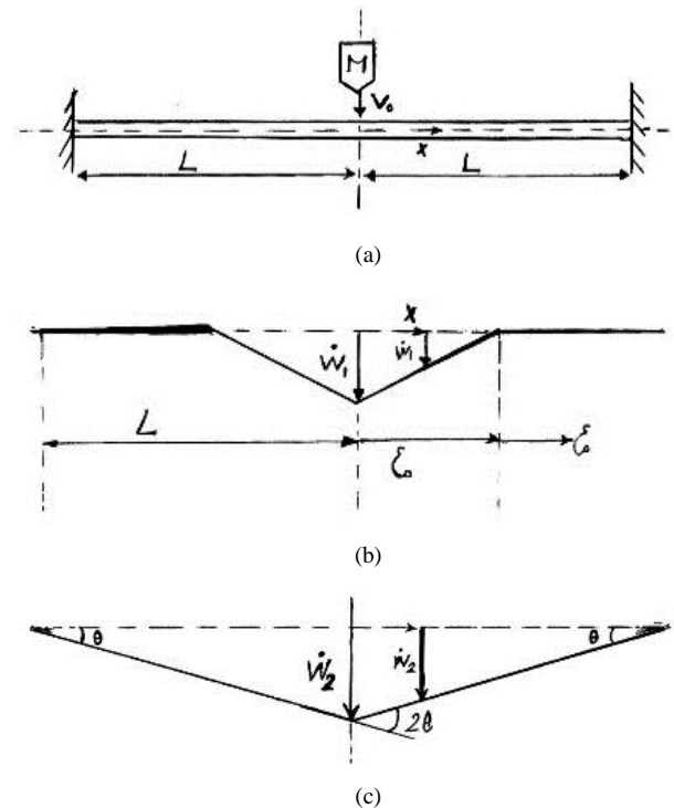
Figure 7. (a) Stroke of mass ( M ) with initial velocity of V with fixed beam, (b) Index of transverse velocity for first phase of motion, 0 \leq t \leq t_1 , (c) Index of transverse velocity for second phase of motion t_1 \leq t \leq T
