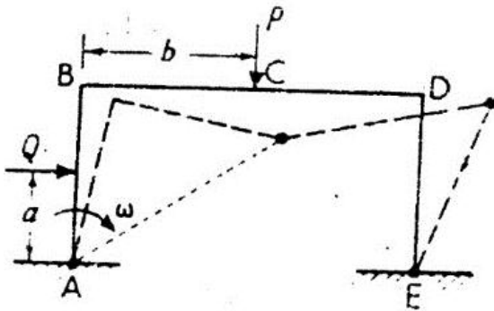
Figure 6. A frame under a vertical load (p) and a horizontal load (Q)
