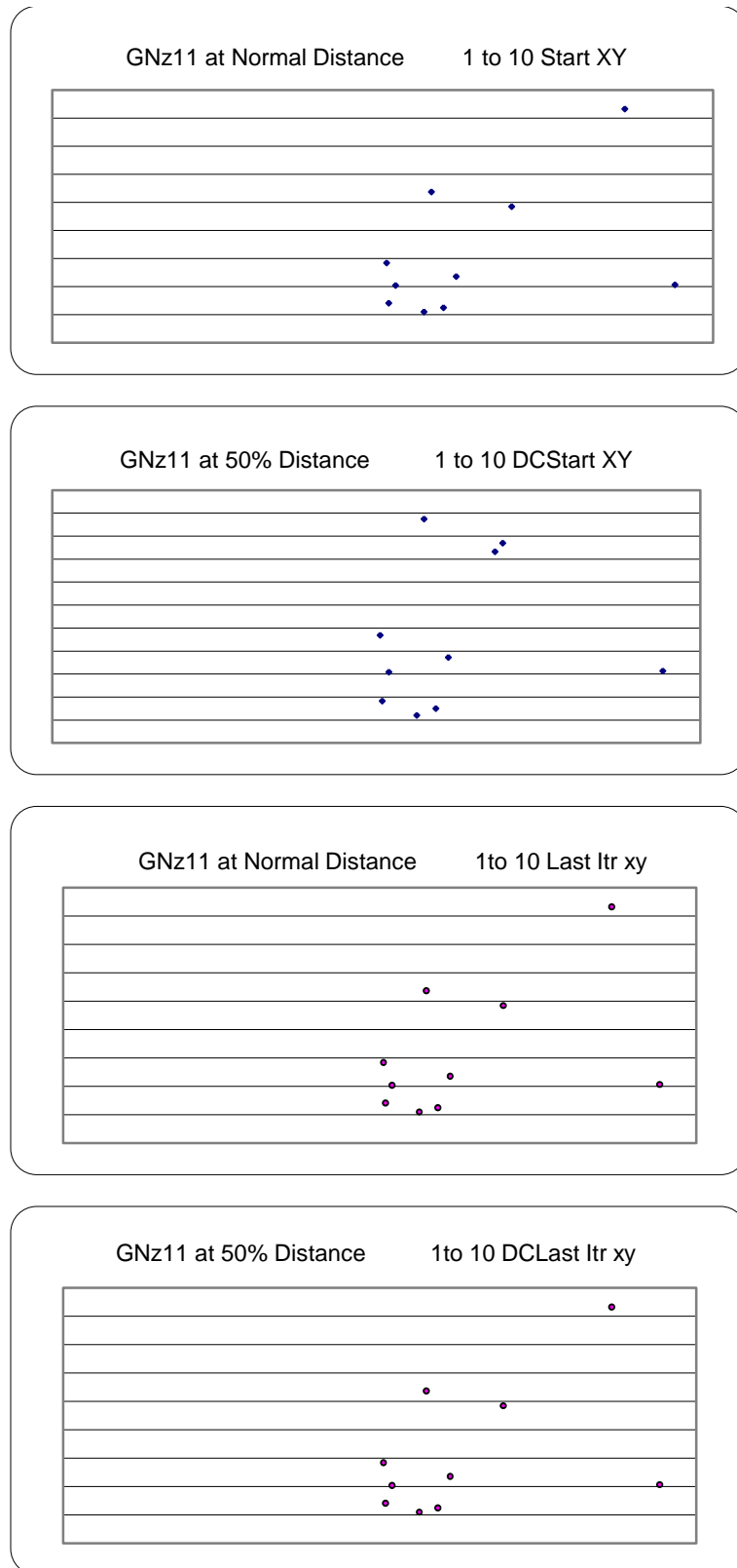
Figure 2. Contains graphs of starting positions and last positions of first 10 Galaxies used in this simulation that is including GNz11. Only these graphs are shown here due to page length constraint and to visualize the exact differences between all these 4 graphs. On can very easily see that the graph named ' 1 to 10 DC start XY ' is different from all the others , which is showing the starting position of GNz11 changed by 50% . And also it may please be noted that SCALES in these start graphs are different to accommodate more clear view.
