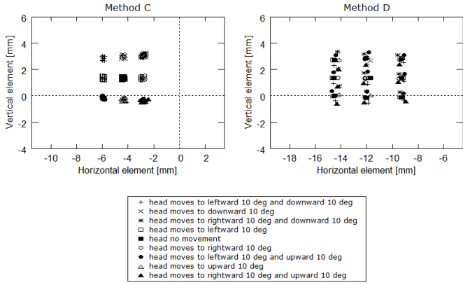
Figure 3. The coordinates of p_{cor} associated with p_{gaze} under an influence of a head movement in Method C and D
