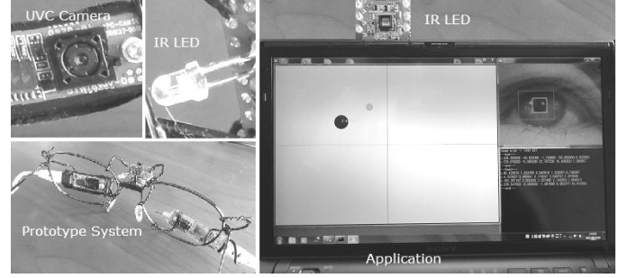
Figure 4. Experimental system
