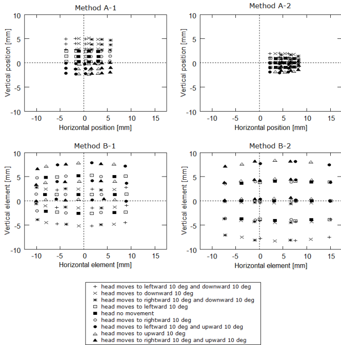
Figure 2. The coordinates of p_{cor} associated with p_{gaze} under an influence of a head movement in Method A and B
