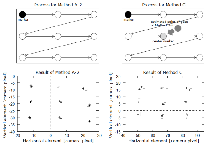
Figure 5. Calibration process and calibration results of Method A-2 and Method C
