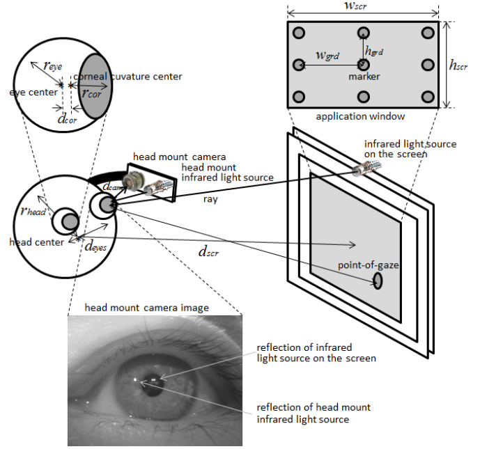
Figure 1. Eye tracking system diagram
