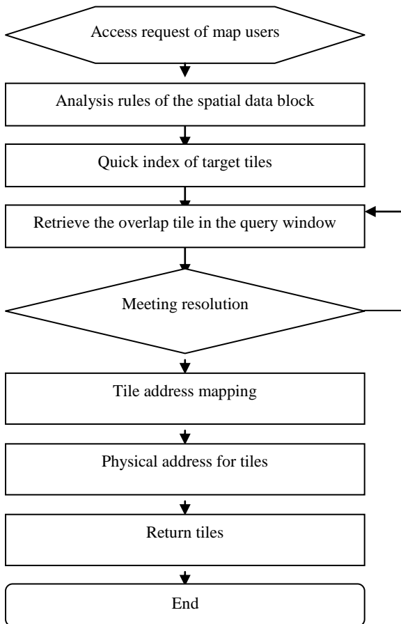
Fig.4 Quick access mechanism based on Quadtree tiles method
