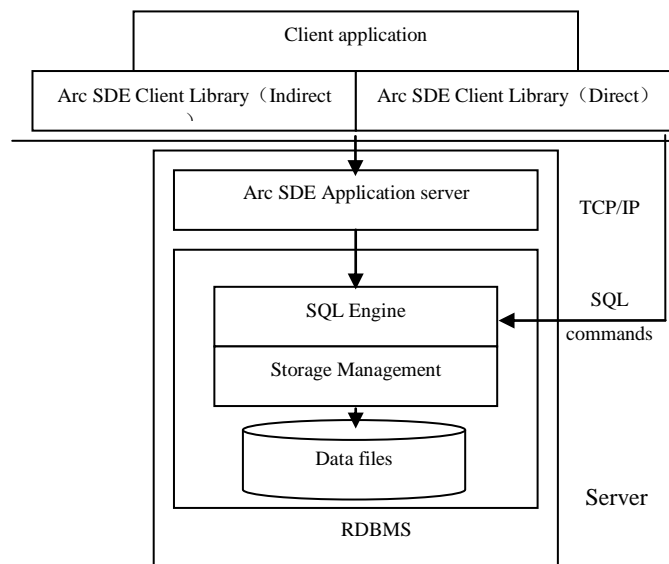
Fig.2 Structure of Arc SDE system
